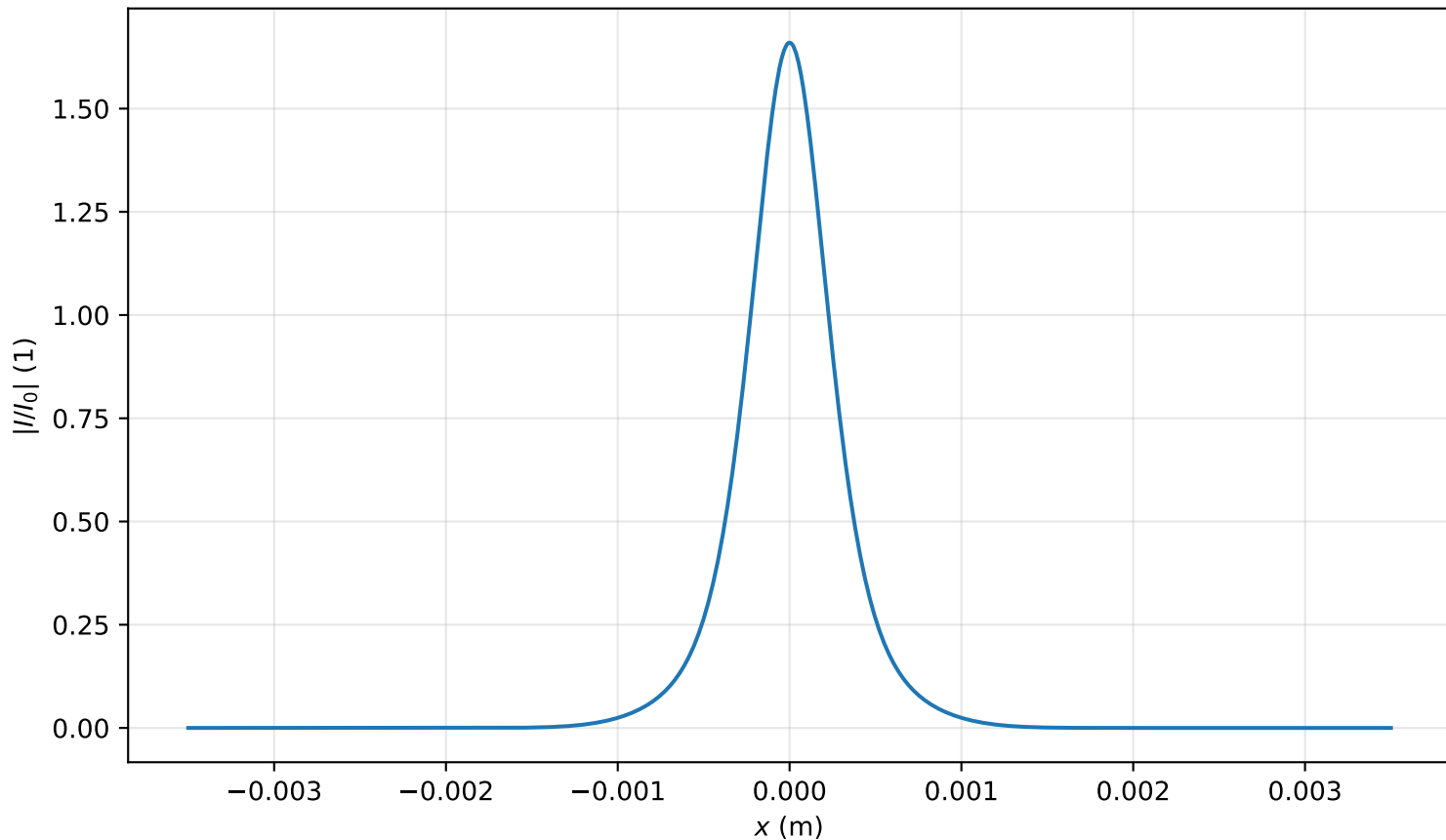
Intensity profile I(x, y = 0, z = 1.194m)/I_0 , P_{in}=1.0P_{cr} , artificial time
